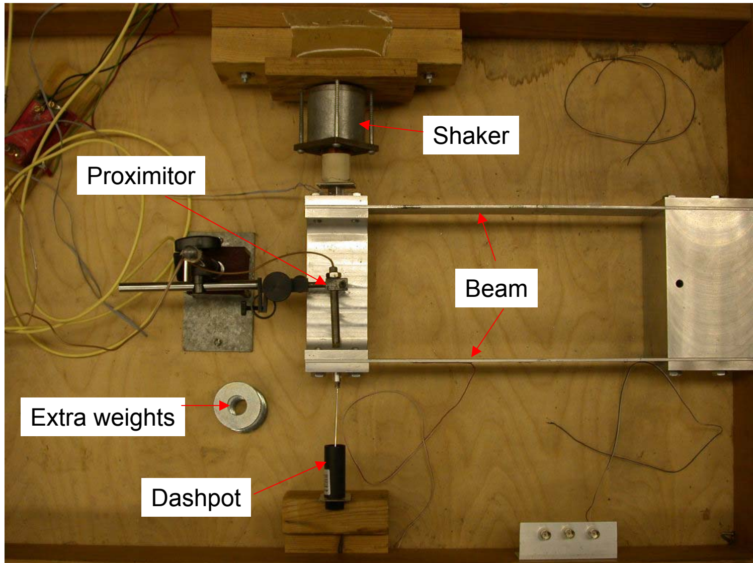
Experiment 6 : Dynamic Response of a Beam Inventory Photos (Not shown : weighing machine (uses the same as in exp. 2))
